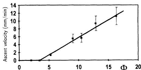
FIG. 4. Ascent velocity of intruders as a function of diameter ratios \Phi at \Gamma=1.25 .
