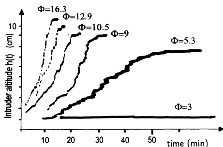
FIG. 3. Ascent diagrams h(t) at \Gamma=1.25 for a set of different diameter ratios \Phi .
