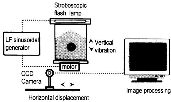
FIG. 1. Sketch of the experimental setup.
